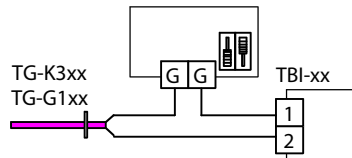
External separate sensor and potentiometer TBI-XX as setpoint
