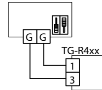
Room control using TG-R4XX as sensor and setpoint
